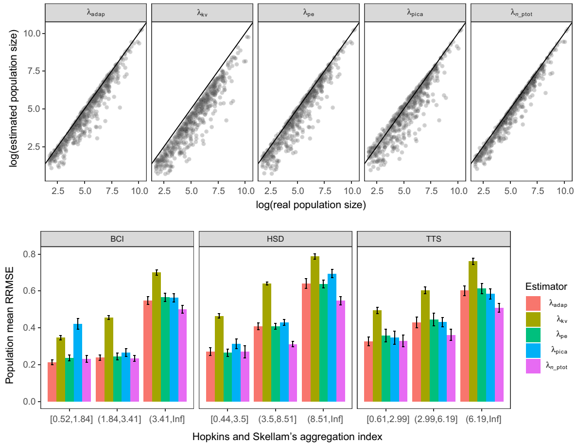
FIG. 4. Performance of our best-performing negative binomial distribution (NBD) estimator ( \lambda_{n\_ptot} ) and other existing estimators for non-CSR population: the \lambda_{pe} estimator (Persson 1964), the \lambda_{kv} estimator (Kleinn and Vilčko 2006), the best \lambda_{adap} estimator (Magnussen et al. 2012), and the \lambda_{pica} estimator (Picard and Bar-Hen 2007) for real tree populations in the three forest plots (Barro Colorado Island [BCI], Heishiding [HSD], and Tiantongshan [TTS]). The top-row panels show the real population densities against the estimated population density for the five estimators. The bottom-row panels show the group mean RRMSEs of the estimators with one standard error bar against the groups of the Hopkins and Skellam (1954) aggregation index of the species distribution. [Color figure can be viewed at wileyonlinelibrary.com ]
