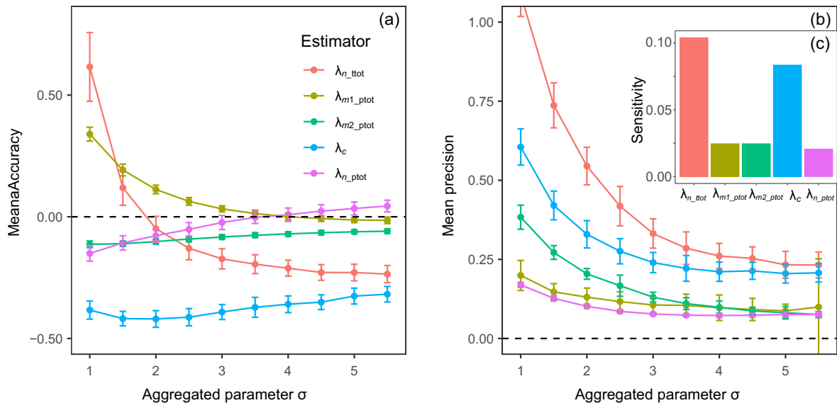
FIG. 2. Performance of the five population density estimators, \lambda_{m1\_ptot} , \lambda_{m2\_ptot} , \lambda_c , \lambda_{n\_ptot} and \lambda_{n\_ttot} (see Table 1 for the notation), for simulated populations varying from high (small \sigma ) to low (large \sigma ) aggregation. Performance of each estimator was presented by plotting (a) the averaged accuracy, (b) precision against aggregation parameter \sigma , and (c) sensitivity across sample size over 99 repeated simulated populations. Vertical bar at each solid point is one standard deviation. Note Eqs. 2 and 3 are indefinite at l = 1 and lq = 1 , respectively; the performance shown here was based on distances at least to the second nearest tree ( l \geq 2 ). Performance of all estimators, except \lambda_{m1\_ptot} , for distances ( lq \geq 2 ) is given in Appendix S4. [Color figure can be viewed at wileyonlinelibrary.com]
