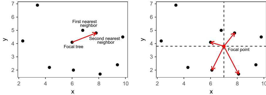
FIG. 1. Illustrating the general distance sampling scheme. On the left panel, distance is sampled from a randomly selected tree (i.e., a tree represented by a black dot) to its second nearest neighbor. On the right panel, distances are sampled from a random point (i.e., an empty location represented by a red dot) to its first nearest-neighbor tree in each of the four equal angle sectors. In the first case, q = 1 and l = 2 ; in the second case, q = 4 and l = 1 . [Color figure can be viewed at wileyonlinelibrary.com ]
