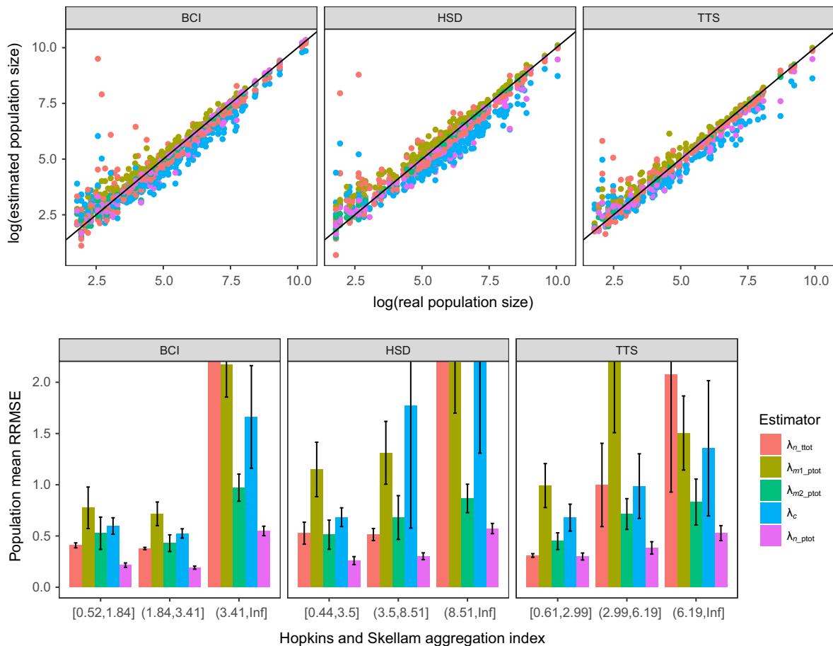
FIG. 3. Performance of the five estimators ( \lambda_{m1\_ptot} , \lambda_{m2\_ptot} , \lambda_c , \lambda_{n\_ptot} and \lambda_{n\_tot} ; see Table 1 for notation) for real tree populations in the Barro Colorado Island (BCI), Heishiding (HSD), and Tiantongshan (TTS) plots. The top-row panels show the real population densities against the estimated population density. The bottom-row panels show the group mean RRMSEs of the estimators with one standard error bars against the groups of the Hopkins and Skellam (1954) aggregation index for the species examined. The aggregation of species distribution increases with the group values from left to right. [Color figure can be viewed at wileyonlinelibrary.com ]
